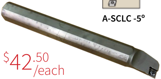
A-SCLCL/R 1" Diameter Boring Bars for CCMT09 inserts
