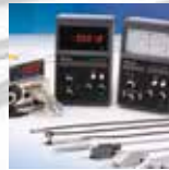
Mu-checker
